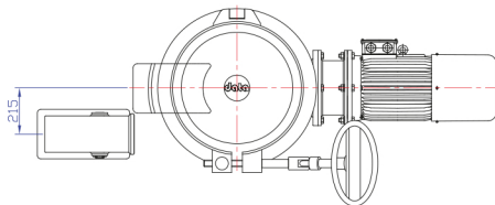
Electric motor drive 90° (380 V)
